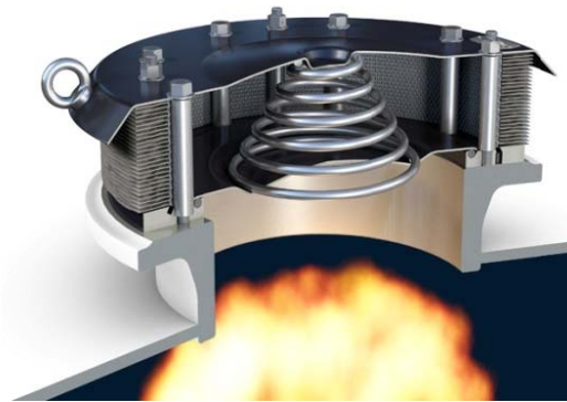
Valve Closed
