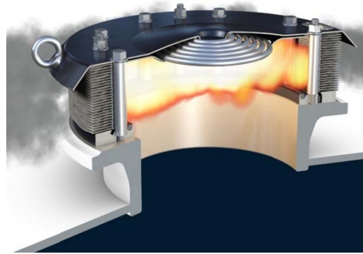
Valve Open
